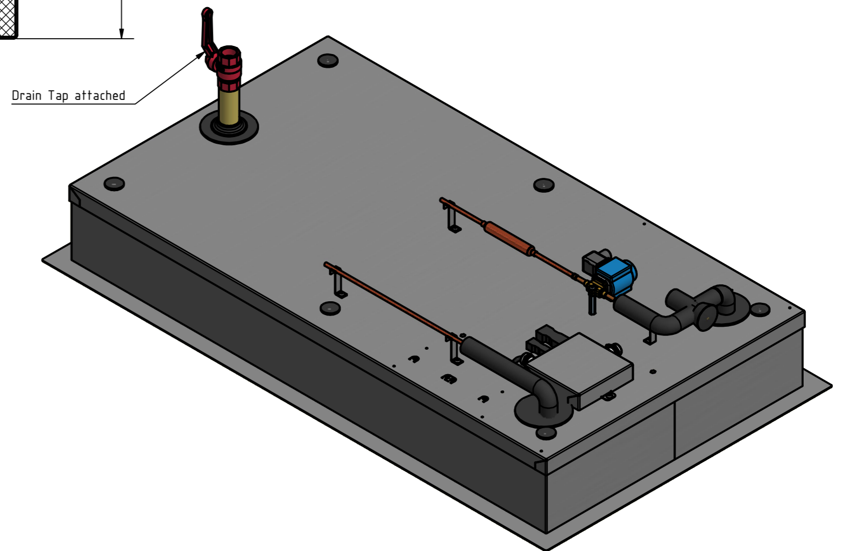
View from below ( 1 : 6 )
